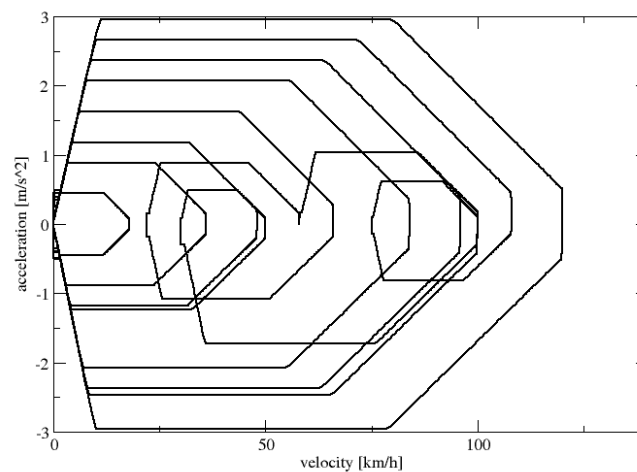
Figure 1 The TNO Dynacycle in terms of velocity and acceleration shows how in particular the hard accelerations and decelerations are covered. Some vehicle are not able to follow the hard accelerations (above 2 \text{ m/s}^2 ), and they are instead operated at full throttle.
