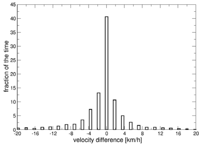
Figure 20 The time shares of velocity differences with the car in front from the radar data. More than 40% of the time the velocity difference is smaller than +/- 0.5 m/s, despite the delayed reactions in the case of car following.
